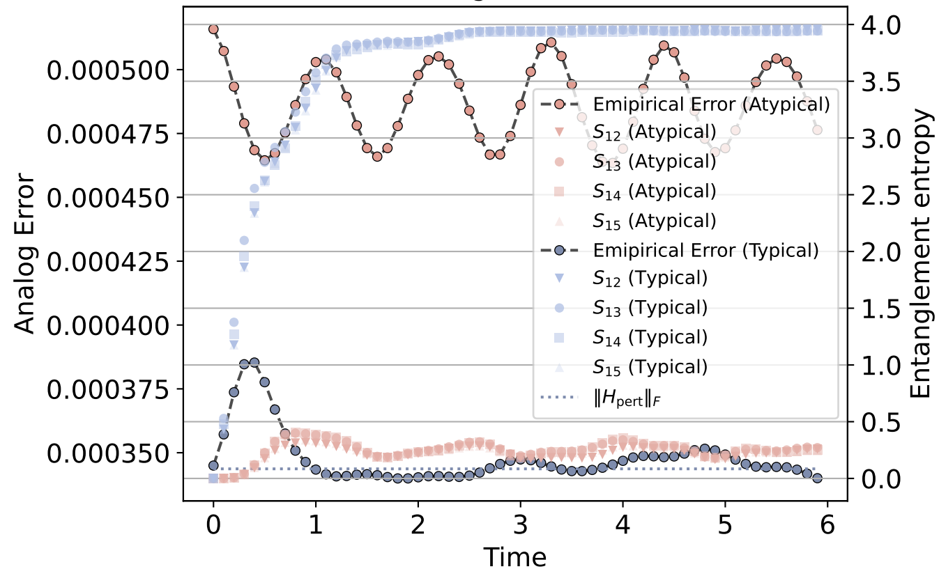
2D-lattice QIMF, one segment evolution with disorder
